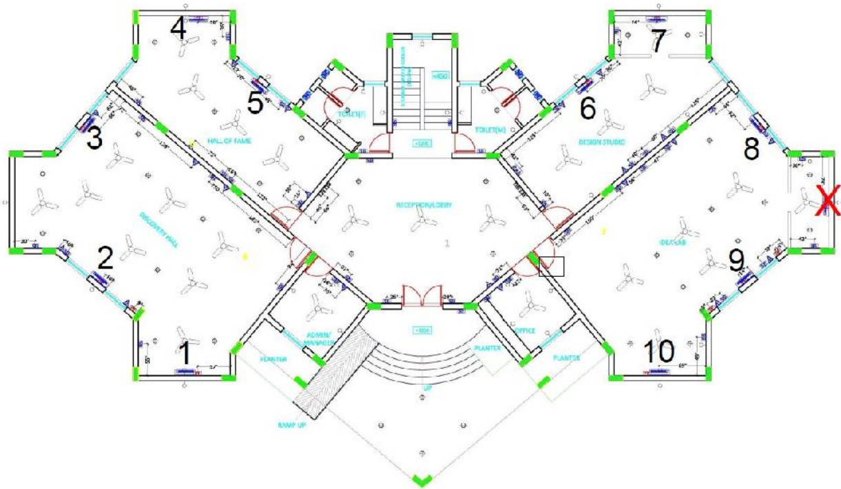
SPLIT AC IDU LOCATION MAP
